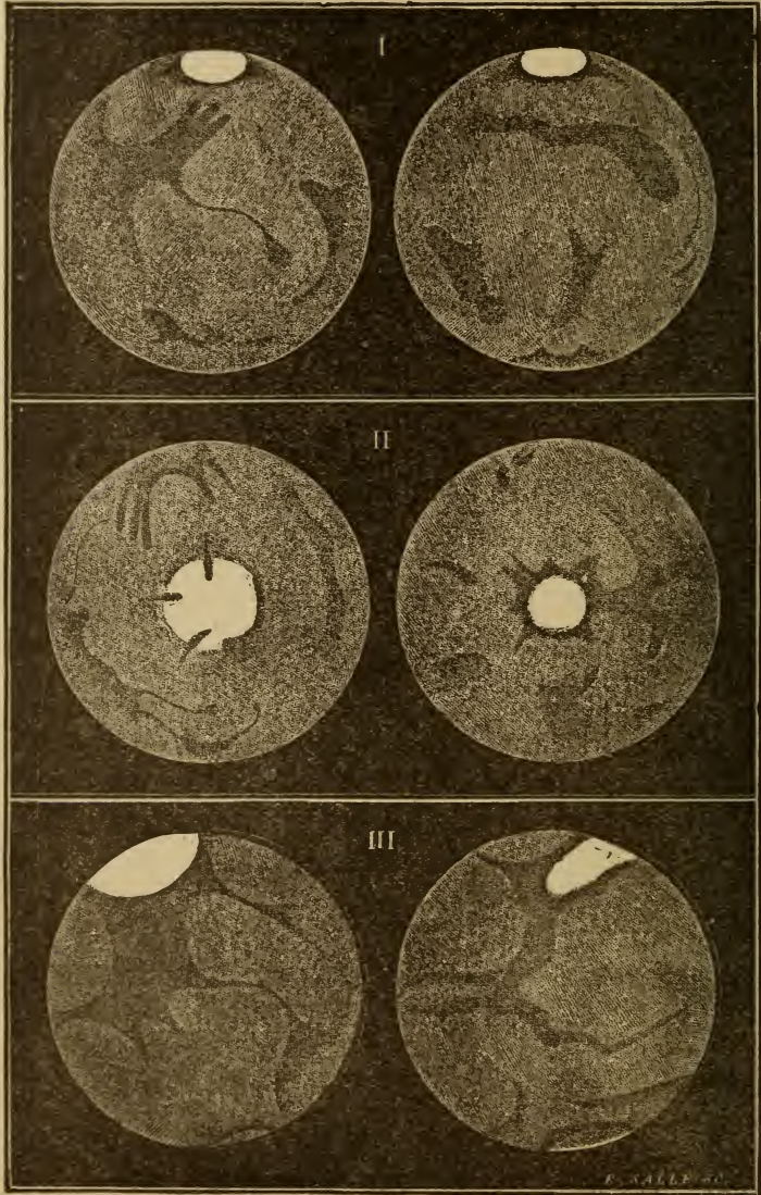
Fig. 173. MARS.
